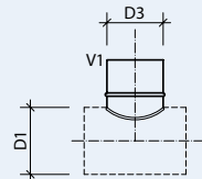
PS/PSU Sattelstück
